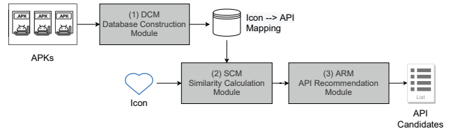
Figure 2: The architecture of Icon2Code .
