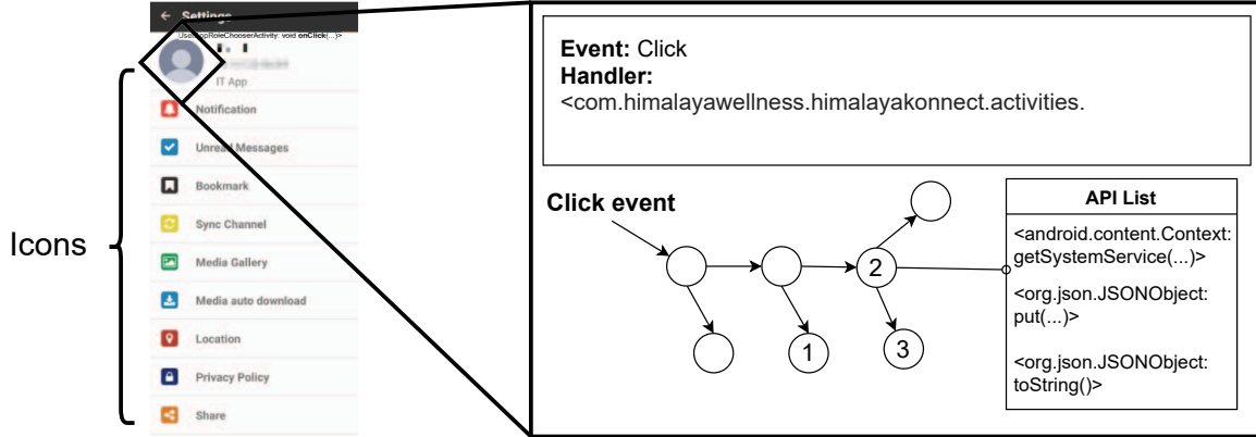
Figure 1: An example of icon-bound GUI components and icon-related event handler callback methods.
